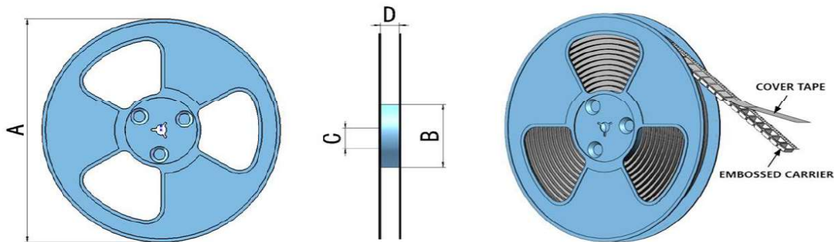
Reel Dimension Schematic Diagram ( mm )
