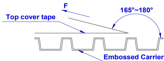
Tearing Off Force Schematic Diagram
