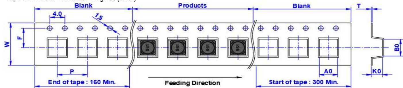
Tape Dimension Schematic Diagram ( mm )
